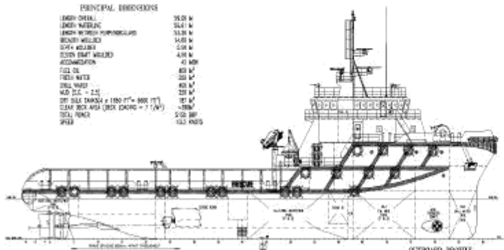
STARBOARD PROFILE
